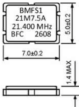
All dimensions are typical unless otherwise specified
